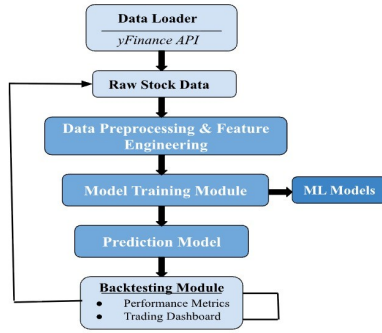
Fig. 1. System Architecture of Proposed Stock Prediction System
